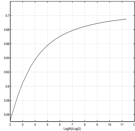
Figure 1: Curve \text{Log}_2(N) \mapsto \sigma_{\max}(\bar{M}) .
